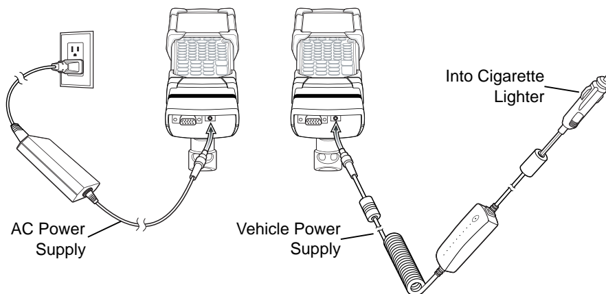
Figure 7-8 MSR Power Connection
