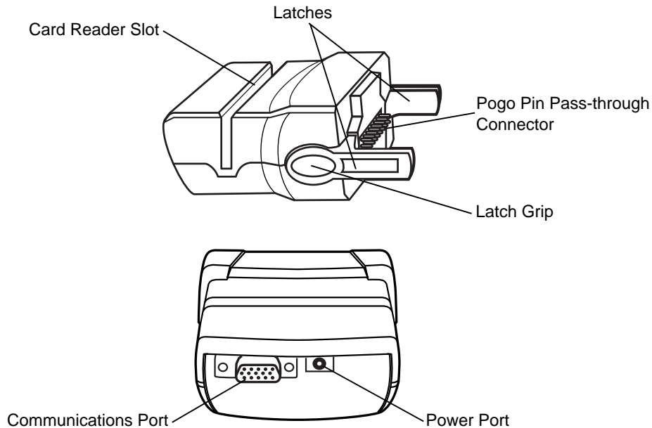
Figure 7-6 Magnetic Stripe Reader
