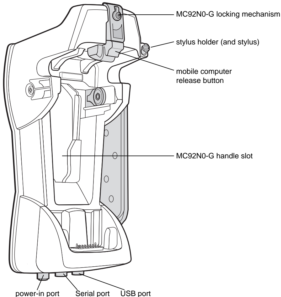
Figure 7-20 Forklift Cradle
