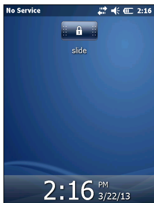
Figure 2-11 Lock Screen
