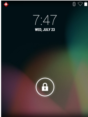
Figure 3-14 Lock Screen
