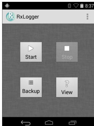
Figure 3-27 RxLogger
