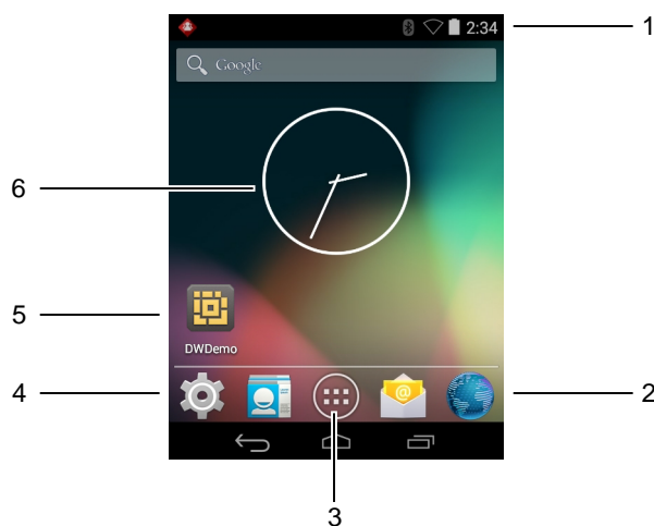
Figure 3-1 Home Screen
