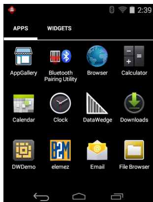
Figure 3-7 APPS Window
