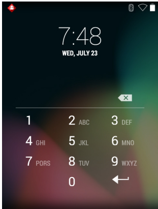
Figure 3-10 PIN Screen
