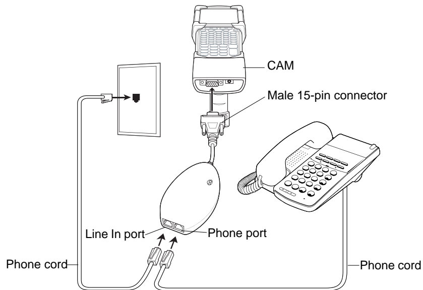
Figure 7-18 Modem Dongle Connection - MC92N0-G
