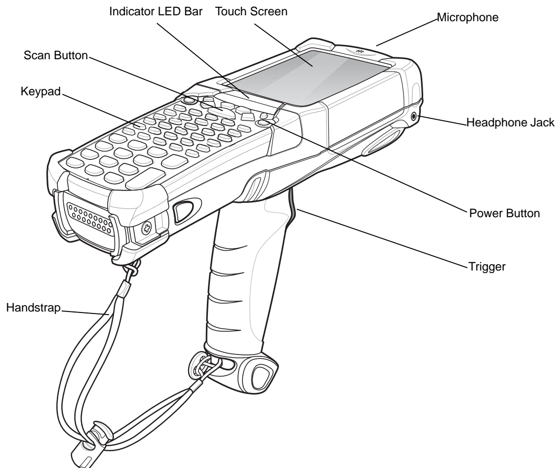
Figure 1-1 MC92N0-G
