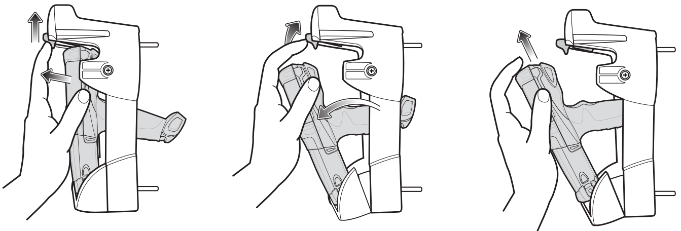
Figure 7-22 Remove MC92N0-G from Forklift Cradle
