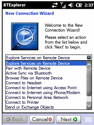
Figure 5-6 BTExplorer Window
