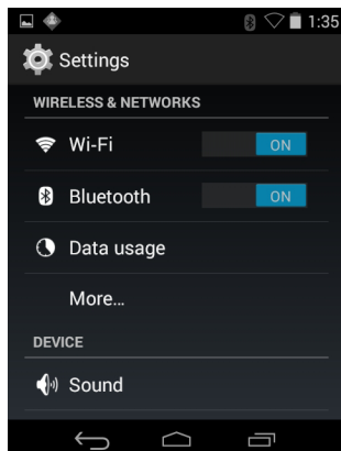
Figure 3-30 Settings Screen
