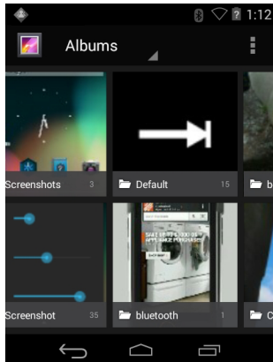
Figure 3-16 Gallery — Albums
