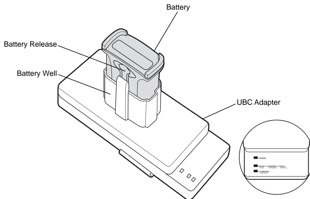
Figure 7-15 UBC Adapter
