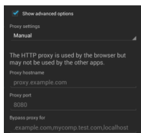
Figure 3-33 Proxy Settings
