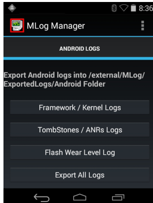
Figure 3-26 MLog Manager
