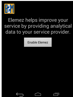
Figure 3-28 Elemez Application
