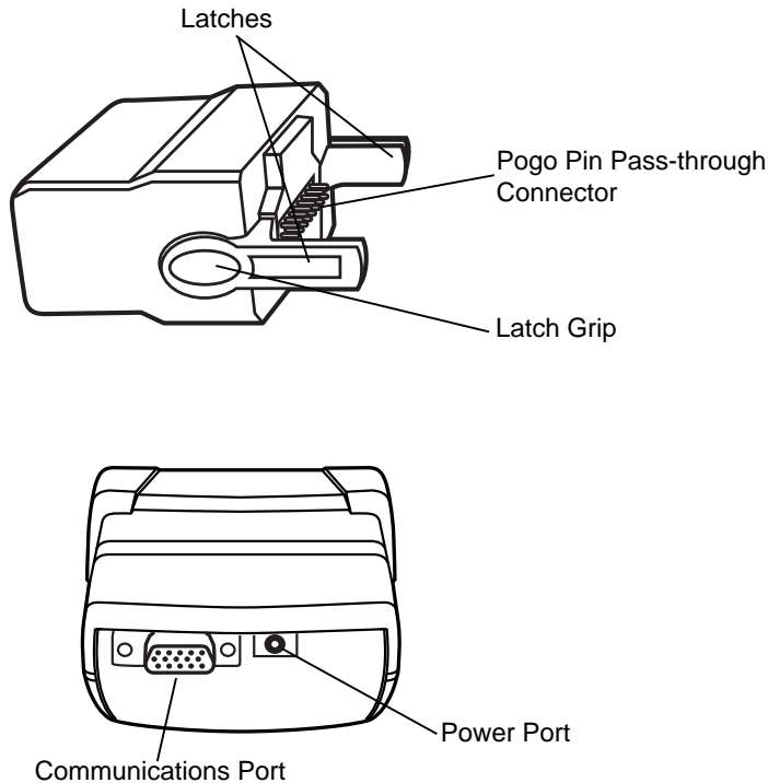
Figure 7-11 Cable Adapter Module
