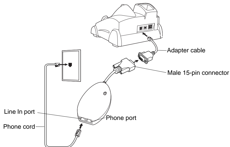
Figure 7-19 Modem Module Connection - Single Slot Serial/USB Cradle
