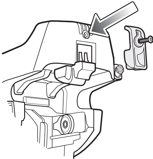
Figure 7-23 Locking Mechanism
