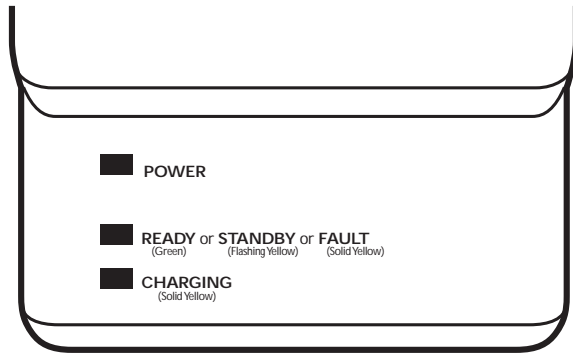
Figure 7-16 UBC Adapter LEDs
