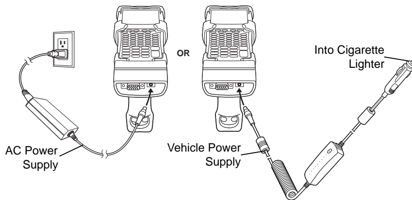
Figure 7-13 CAM Power Connection
