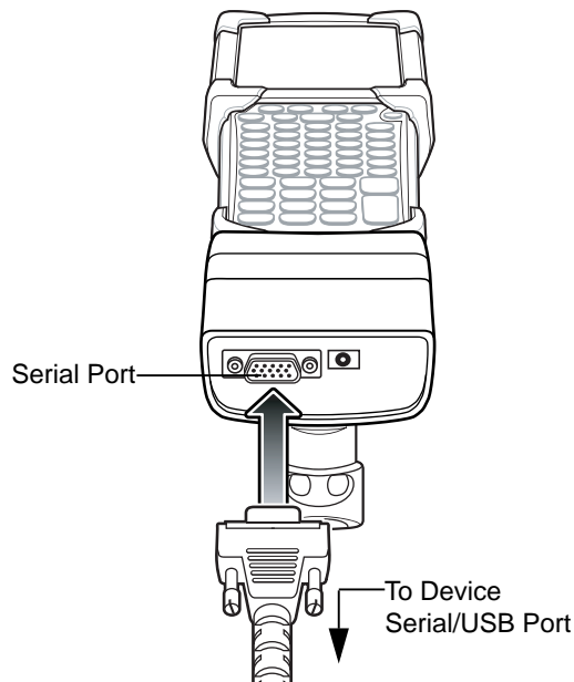
Figure 7-14 CAM Serial Connection
